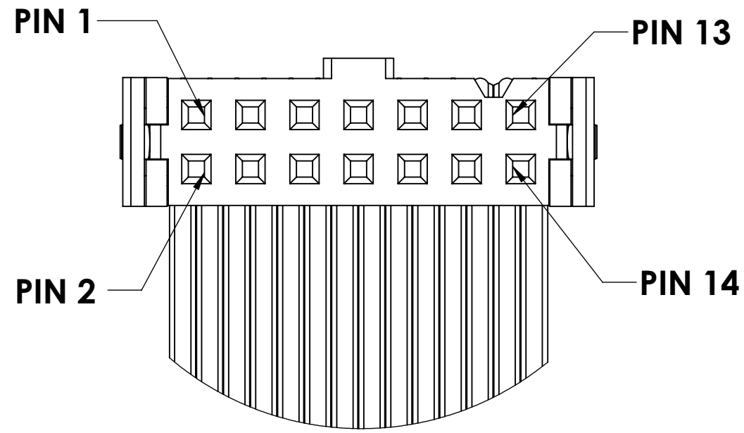
DETAIL F SCALE 4 : 1
